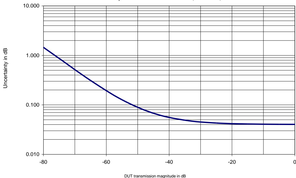
Transmission magnitude uncertainty with the R&S®FSH13 model .23/R&S®FSH20 model .30.
