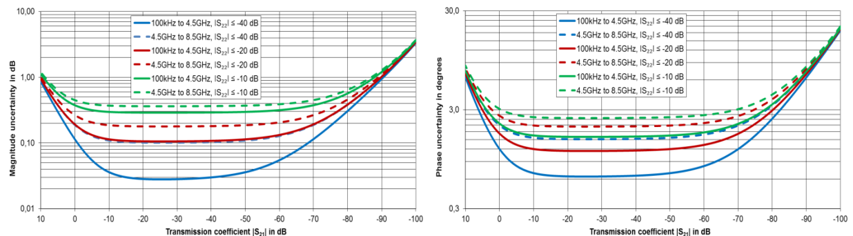
Typical accuracy of transmission magnitude and transmission phase measurements for the R&S®ZND Analysis conditions: S_{11} = 0 , cal. power -10 dBm, meas. power -10 dBm, base unit or R&S®ZND-K1 installed.
