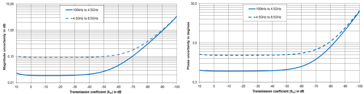
Typical accuracy of transmission magnitude and transmission phase measurements for the R&S®ZND Analysis conditions: S_{11} = S_{22} = 0 , cal. power -10 dBm, meas. power -10 dBm, R&S®ZND-K5, R&S®ZND-K6 or R&S®ZND-K8 installed.
