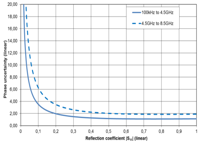
Typical accuracy of reflection magnitude and reflection phase measurements for the R&S®ZND Analysis conditions: S_{12} = S_{21} = 0 , cal. power -10 dBm, meas. power -10 dBm, R&S®ZND-K5, R&S®ZND-K6 or R&S®ZND-K8 installed.
