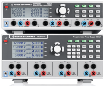
R&S®HMP2030 three-channel and R&S®HMP4040 four-channel power supply
