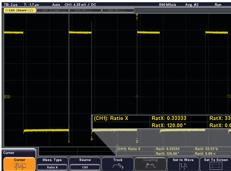
Special cursor measurement: using three cursors to determine the duty cycle of a pulsed signal.
