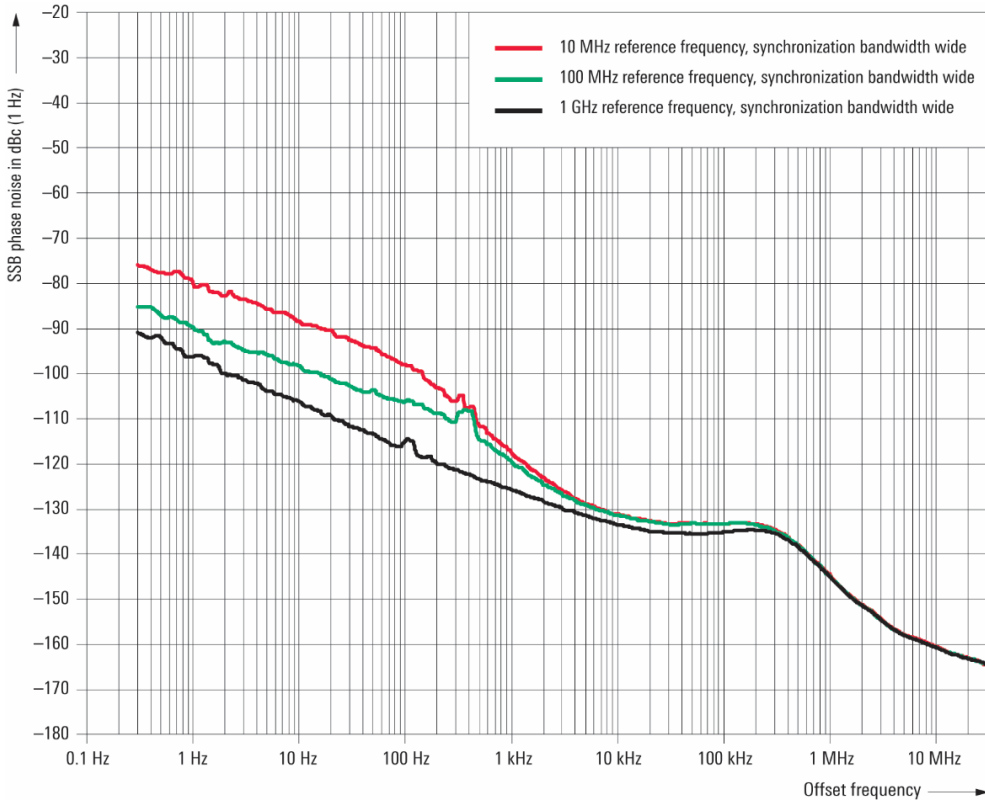
Measured residual SSB phase noise at f = 10 GHz with the R&S ® SMAB-B711 option, comparison of different reference frequencies.
