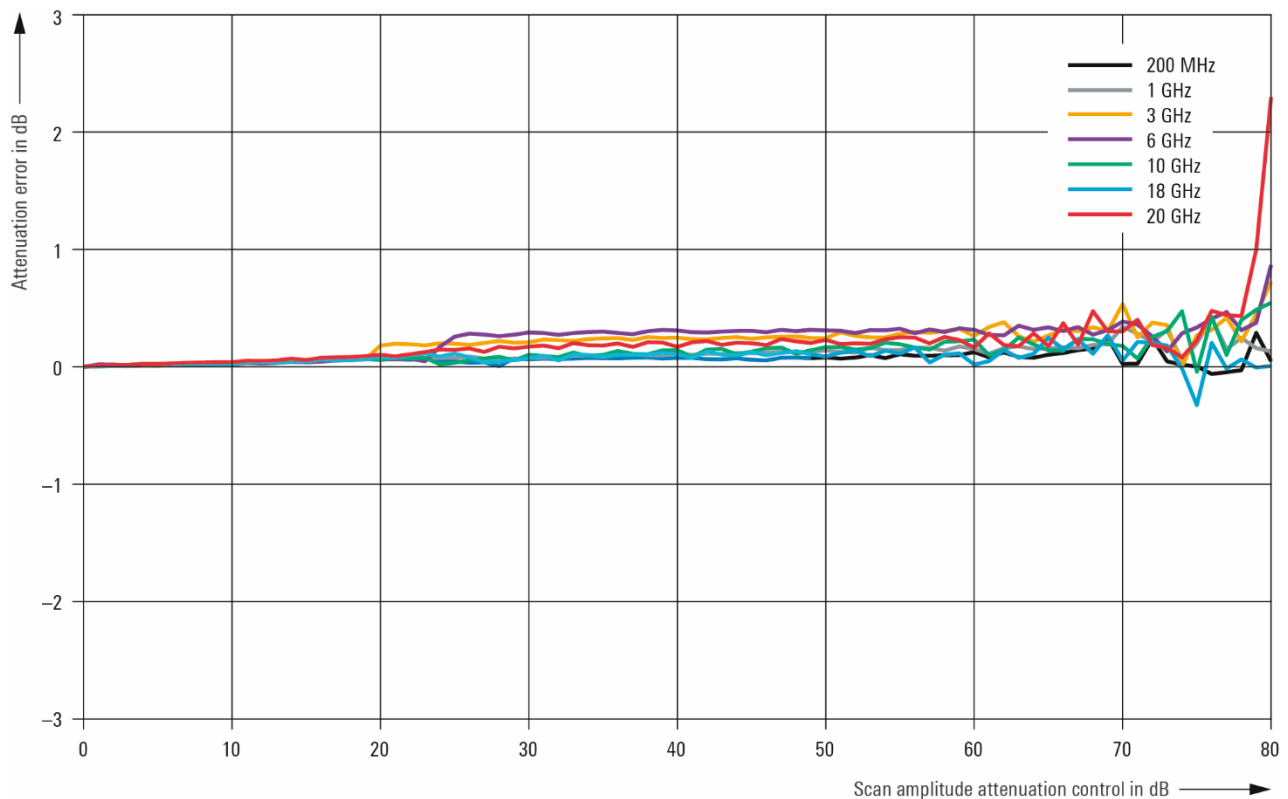
Measured scan AM attenuation error with the R&S®SMAB-K721 option.
