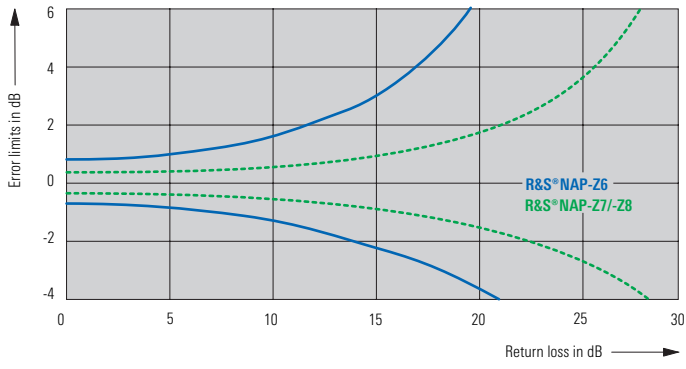
Measurement error limits (two standard deviations) for reflection measurements with the Directional Power Sensors R&S® NAP-Z6, R&S® NAP-Z7 and R&S® NAP-Z8 (with the latter two having a limited frequency range from 1.5 MHz to 30 MHz); min. forward power: see specifications for the power sensors
