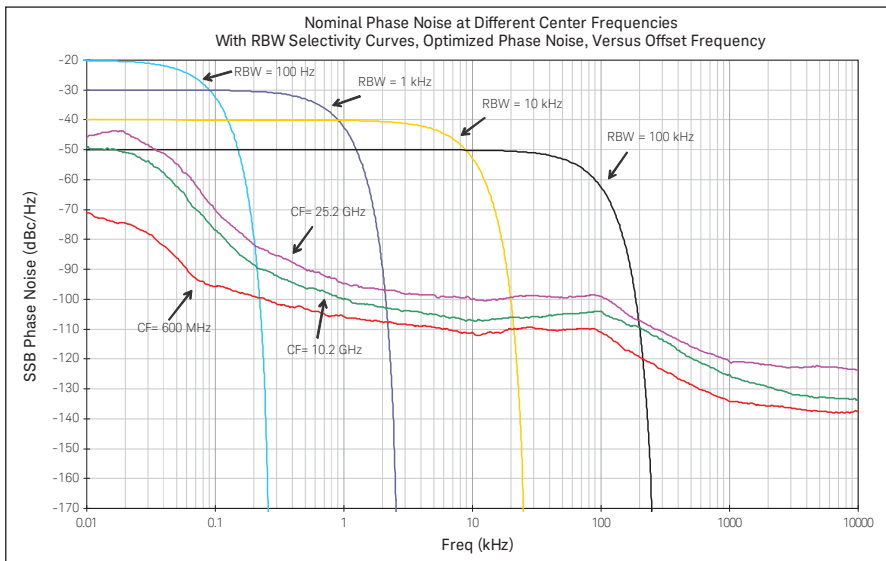
Figure 13. CXA (N9000A) nominal phase noise at different center frequencies
