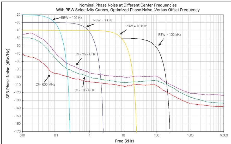
Figure 14. CXA-m (M9290A) nominal phase noise at different center frequencies
