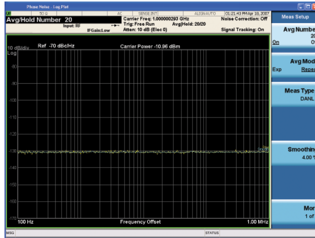
Figure 6. DANL measurement
