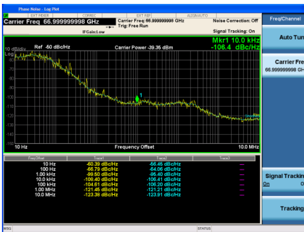
Figure 8. Phase noise measurement at 67 GHz with PXA Option EXM and an external mixer
