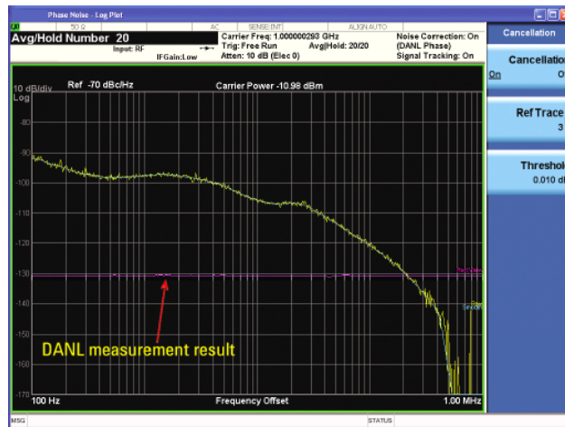
Figure 7. Phase noise plot with subtraction of DANL; the DANL trace is in magenta
