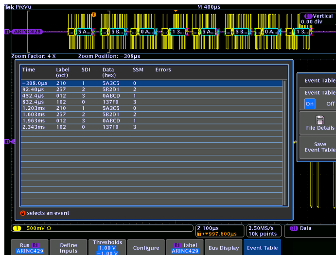
Event table for ARINC 429 bus with all captured packets time stamped and in a tabular view.
