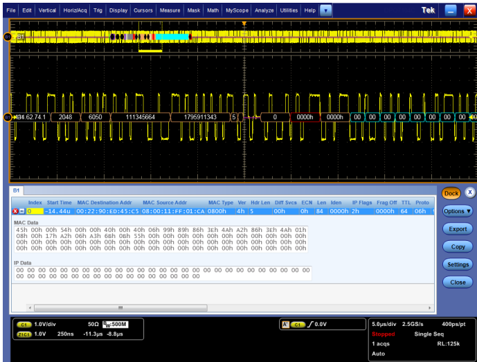
100BASE-TX decoded event table displaying the packet information with time stamp.
